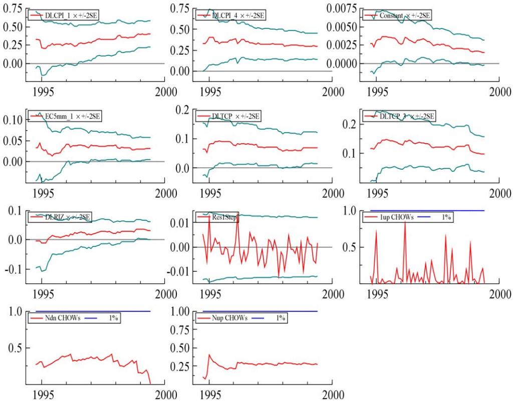
Note. The graphs depict the seven recursively estimated coefficients with two standard errors bands, the one-step ahead residuals, the one-step forecast Chow test (I-up), the break-point Chow test (N-down), and the forecast Chow test (N-up). Details of these tests are found in Hendry and Doornik (2001).
