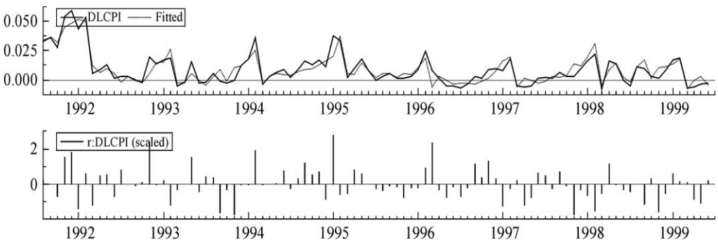
Fig. 3. Actual and fitted values of inflation and the scaled residuals.
